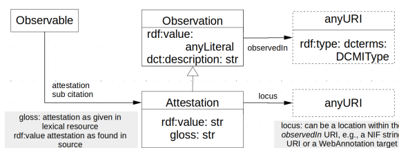
Figure 3: Attestations in OntoLex-FrAC
