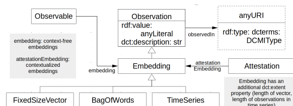
Figure 4: Embeddings in OntoLex-FrAC
