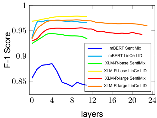
Figure 2: LID model mean F-1 Scores across layers for the probe classifiers. In this task, probe classifiers learn the LID of the tokens in CS sentences.
