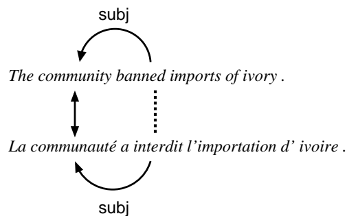
Figure 1: Syntax-based alignment
